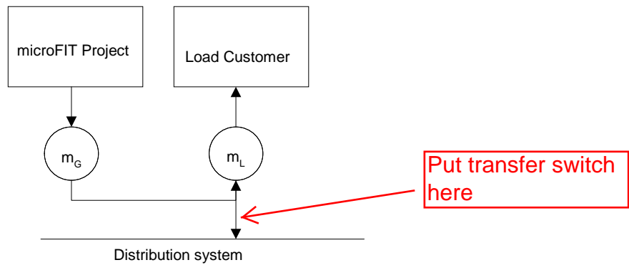
Figure 2 – Indirectly connected microFIT Project (in parallel)
