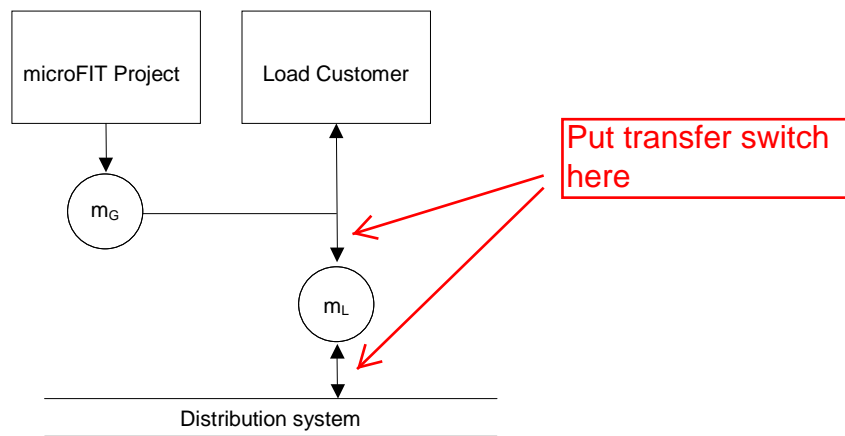
Figure 3 – Indirectly connected microFIT Project (in series)
